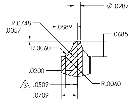
DETAIL B SCALE 8 : 1
