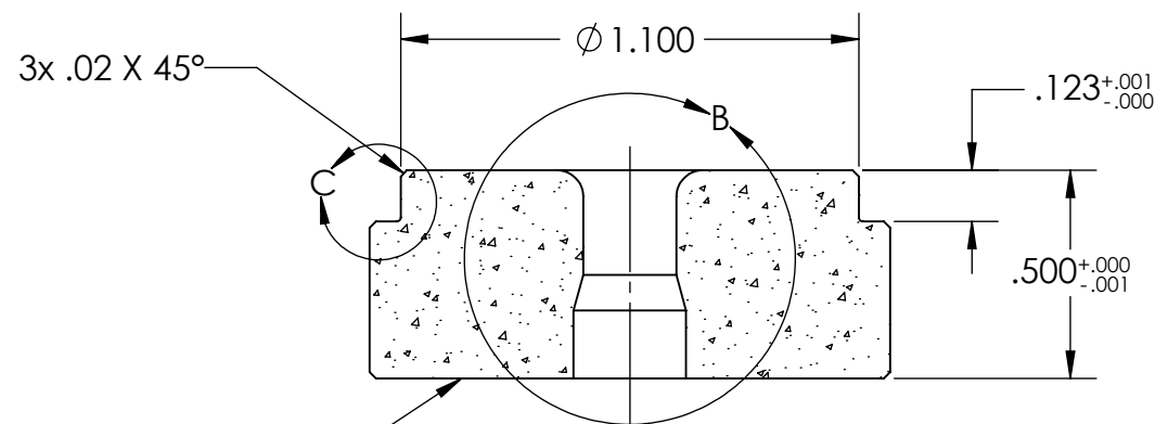
CASED DIE INSERT \phi .750 .004-.006 PRESS FIT
